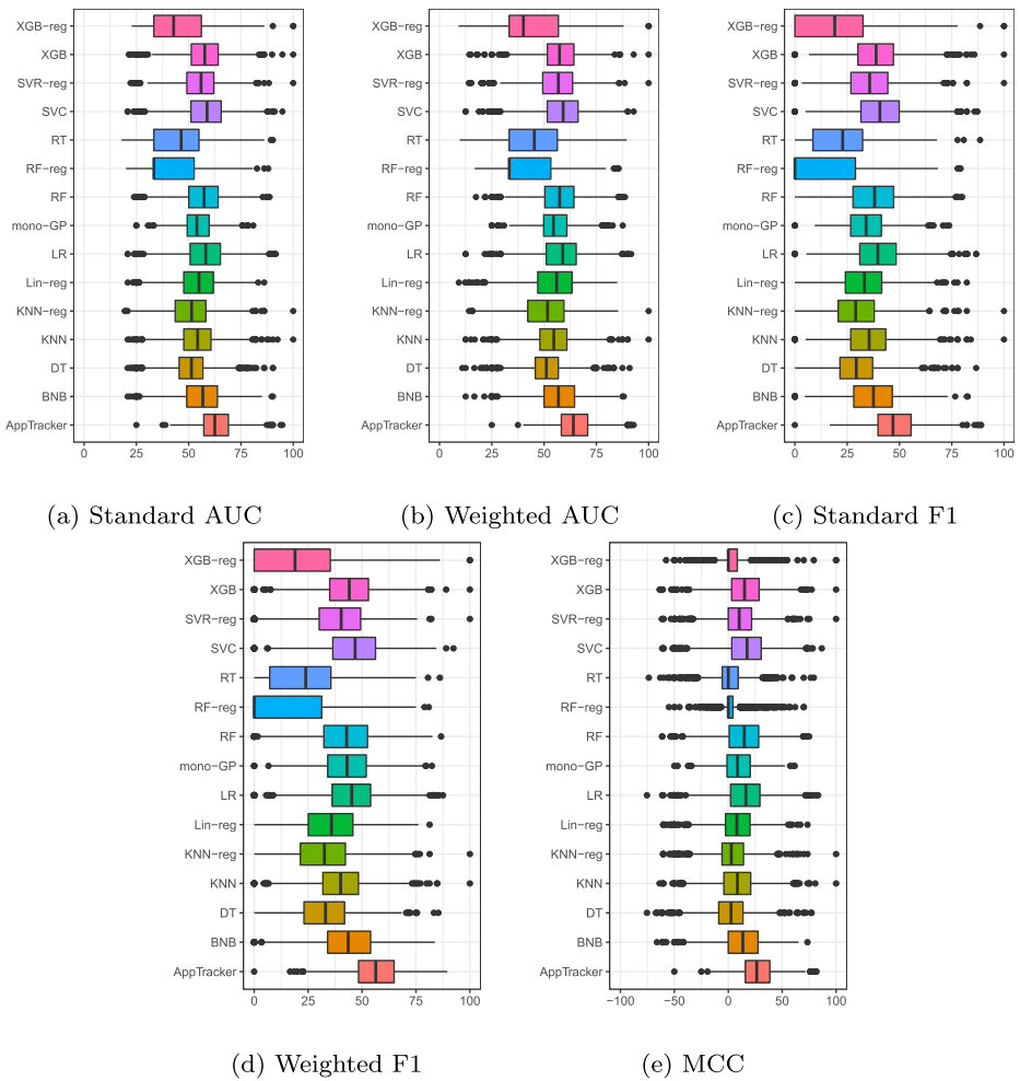
Fig. 12 Boxplots comparing scores of APPTTracker against baseline approaches for cross-project validation
